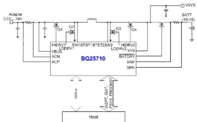
Application Diagram
