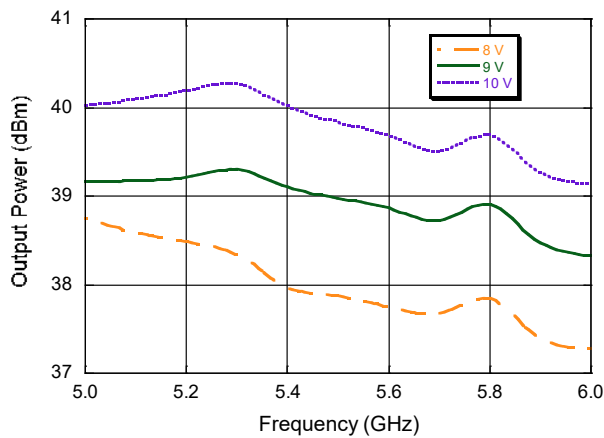
Output Power
