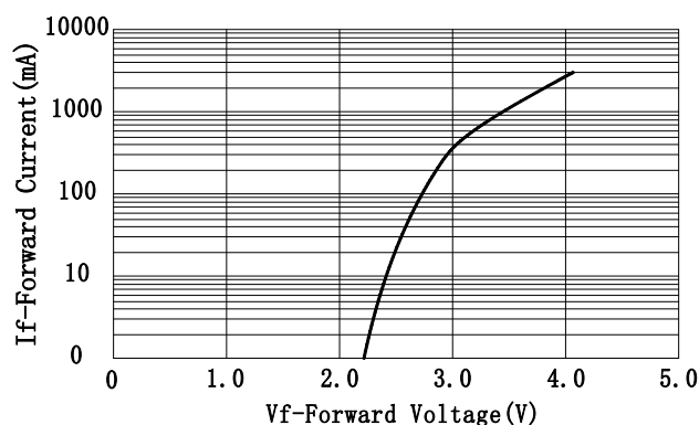
Fig.4-Forward Voltage (@350mA) vs. Temperature
