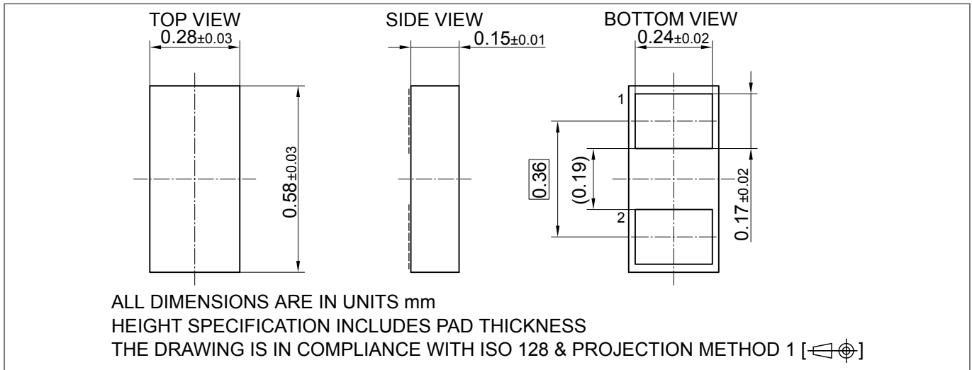
Figure 10 Package outline
