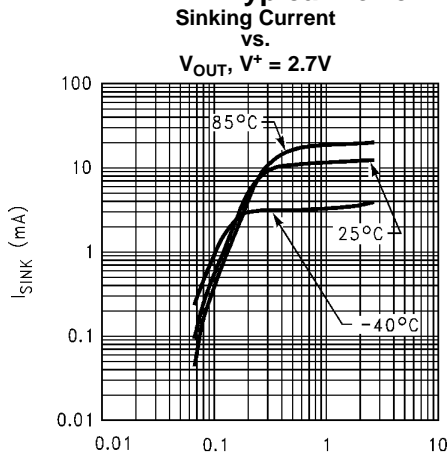
V_{OUT} from V^- (V) Figure 10.
