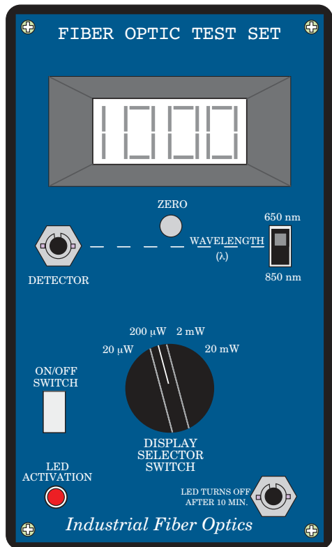
Figure 1. Fiber Optic Test Set front panel
