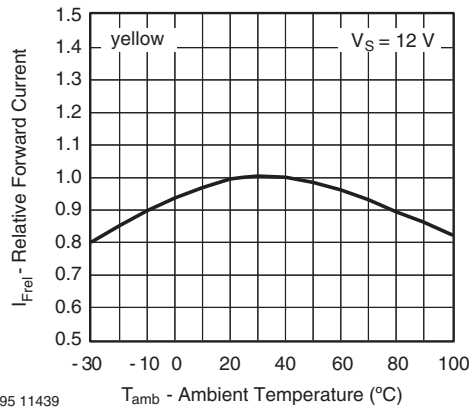
Fig. 14 - Relative Forward Current vs. Ambient Temperature
