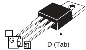
TO-220AB (IXTP)
