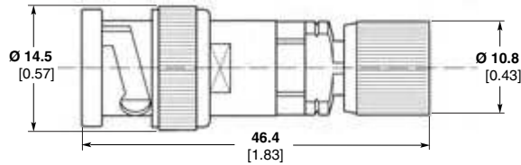
BNC Plug to Plug 1.6/5.6
