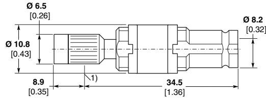
Plug 1.0/2.3 to Jack 1.6/5.6
