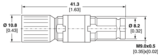
Adapter 1.6/5.6, Plug/Jack
