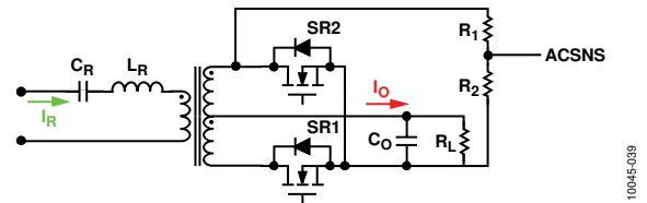
Figure 61. Resonant Synchronous Rectifier Control Circuit
