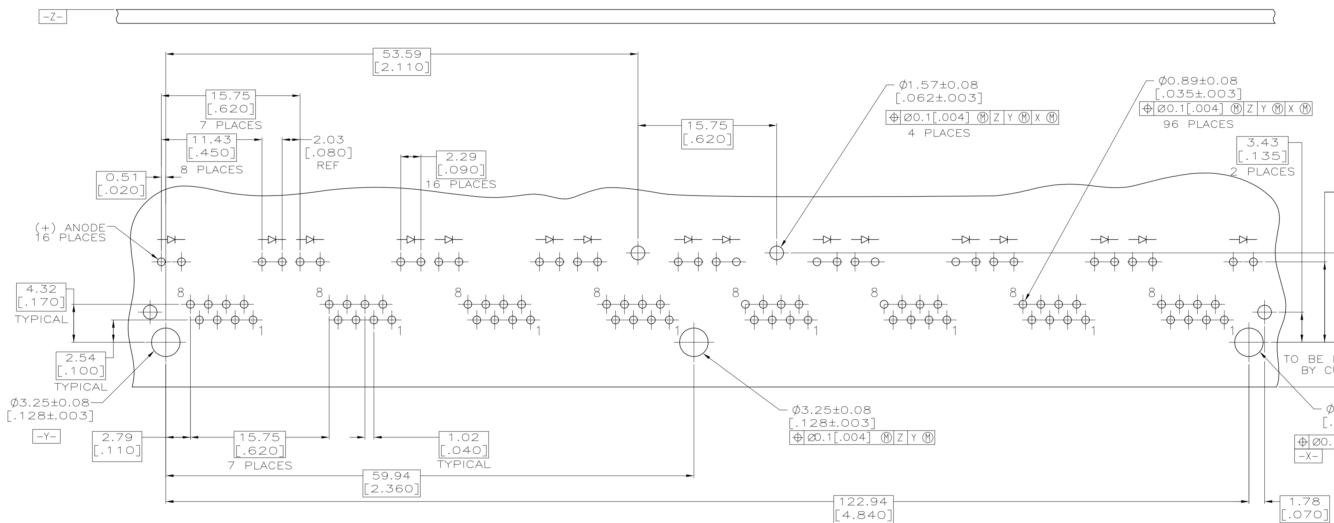
SUGGESTED PRINTED CIRCUIT BOARD LAYOUT (COMPONENT SIDE)
