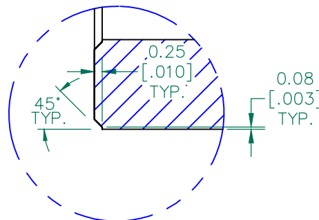
DETAIL "A" CHAMFER SCALE=6:1
