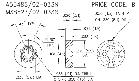
617-075 8 LEADS
