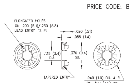
607-075 12 LEADS
