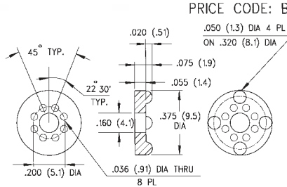
615-075 8 LEADS
