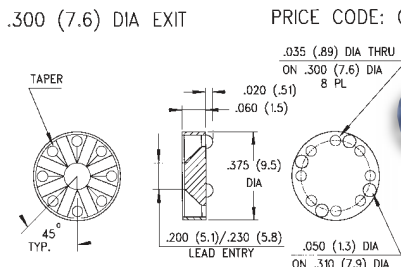
711-085 8 LEADS
