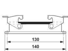
Dimensional drawing
