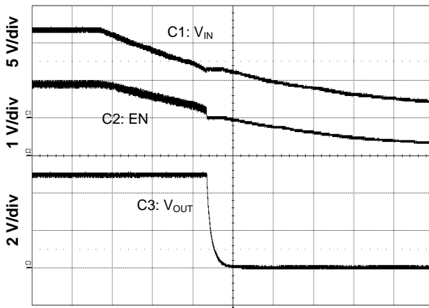
Time = 1 ms/div Figure 18. Shutdown Relative to V_{IN}
