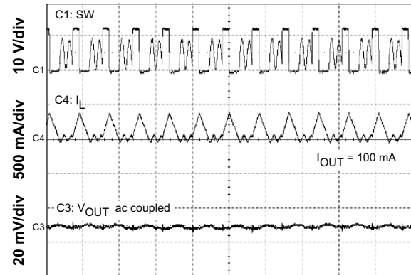
Figure 13. Output Voltage Ripple DCM
