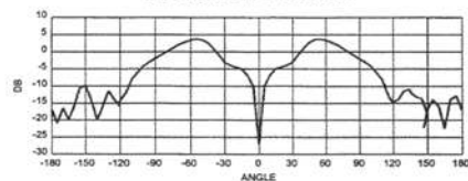
Elevation Pattern
