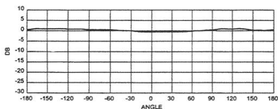
Azimuth Pattern
