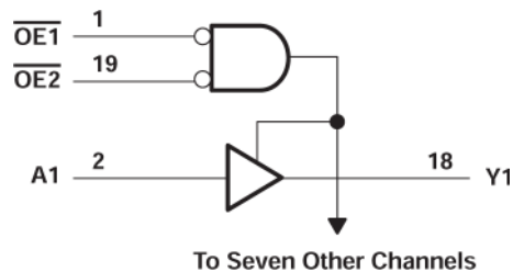
Figure 8-1. Logic Diagram (Positive Logic)
