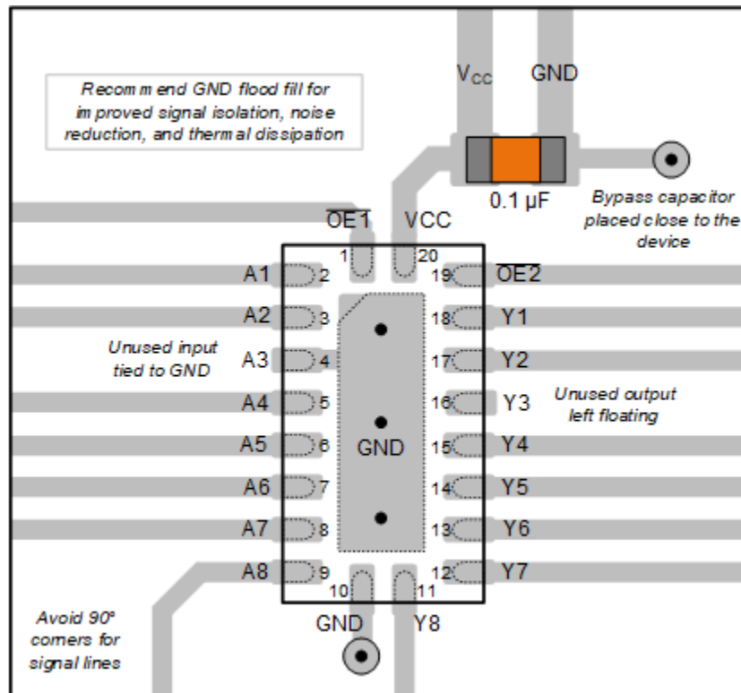
Figure 9-1. Layout Diagram
