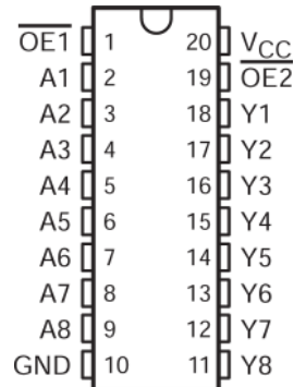
Figure 5-1. D or PW Package (Top View)
