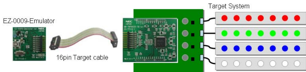
Figure3-4 Connecting EZ-0009-Emulator to Target System
