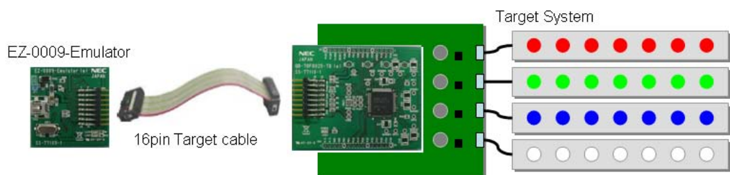
Figure3-7 Connecting EZ-0009-Emulator to Target System
