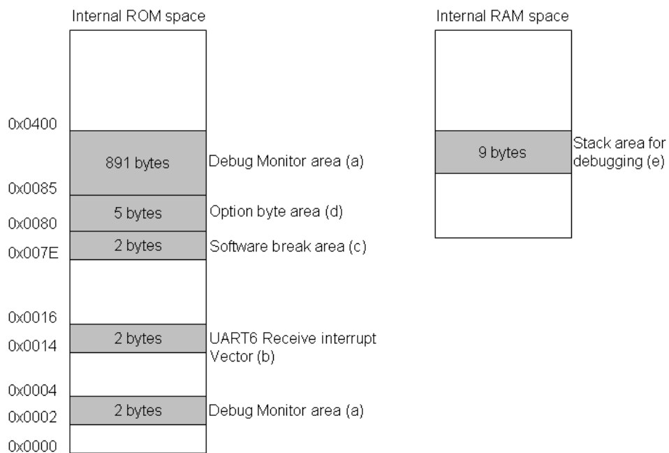
Figure 3-3 Memory spaces Where Debug Monitor Programs are allocated
