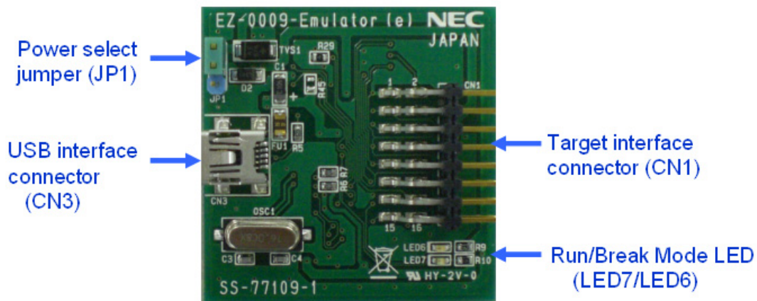
Figure 2-2 Part Names of Simple On-chip debug emulator (EZ-0009-Emulator)
