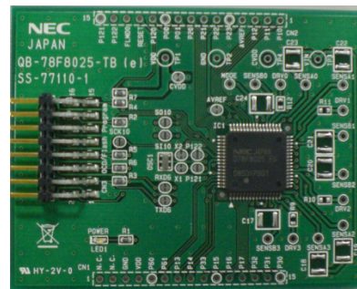
Target board (QB-78F8025-TB)
