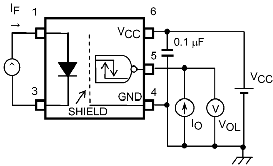
Fig. 12.1.1 V OL Test Circuit
