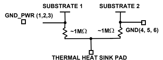
CIRCUIT 6
