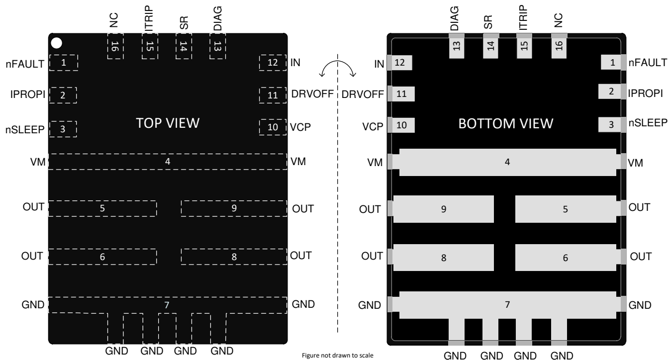
Figure 6-1. DRV8145H-Q1 HW variant in VQFN-HR(16) package
