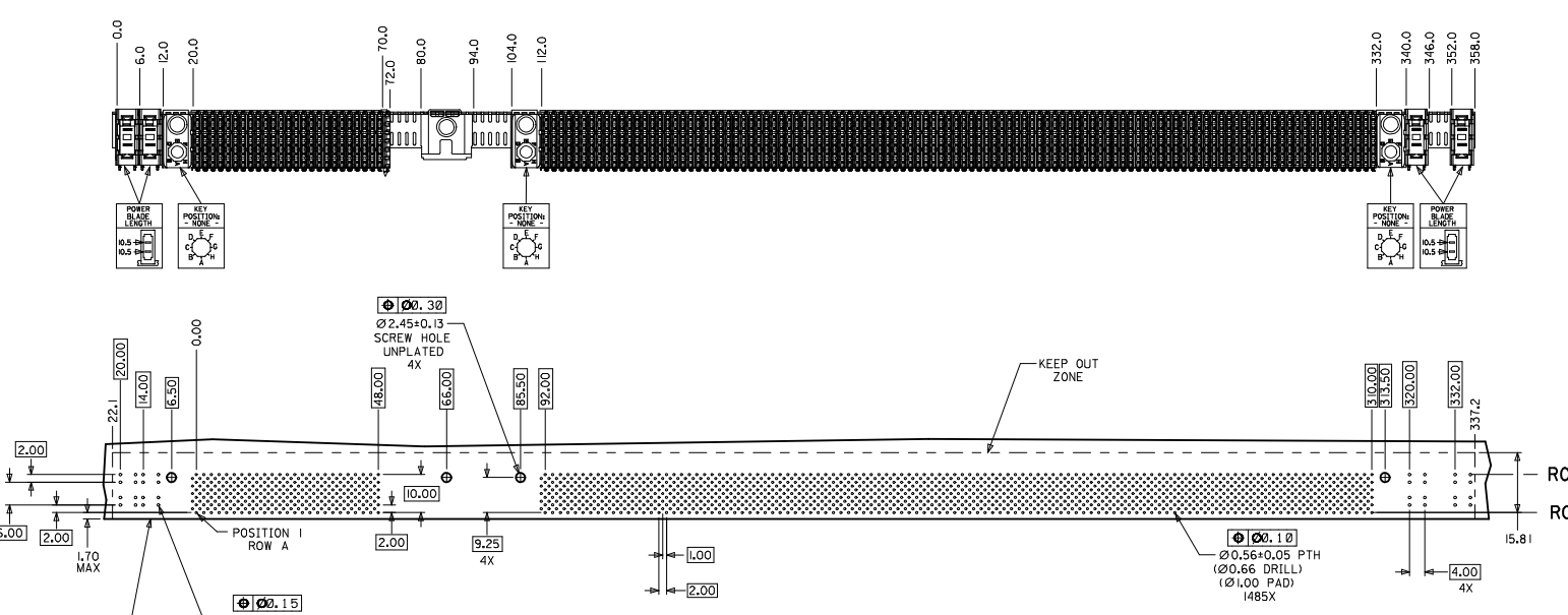
DAUGHTERCARD HOLE PATTERN (CONNECTOR SIDE)
