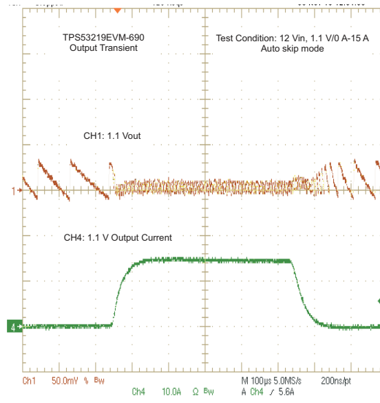
Figure 7-4. Output Load Transient
