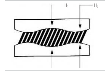
FIGURE 6B. UNEVEN JOINT WITH GASKET
