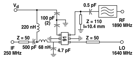
Figure 18. Test Circuit.
