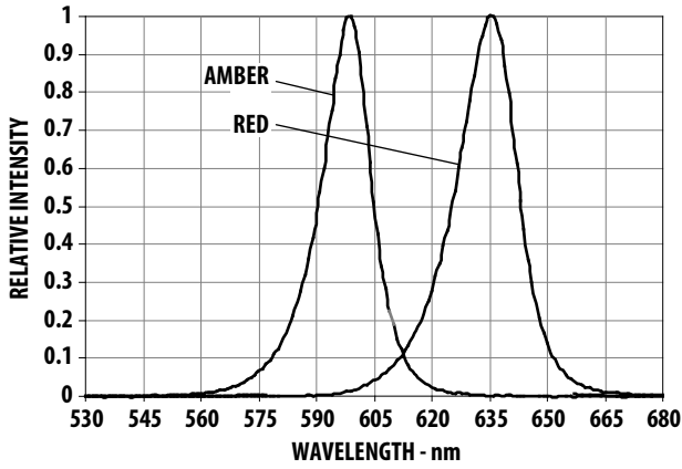
Figure 5 Relative Intensity vs. Wavelength for Red and Amber
