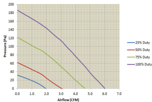
D1U54T-W-800-12-HB3C P-Q Airflow (front to back air direction)
