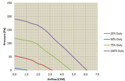
D1U54T-W-800-12-HB4C P-Q Airflow (back to front air direction)
