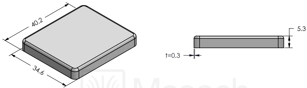
MS402-10S-NS (External Dimensions)
