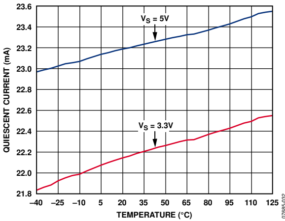
Figure 36. Quiescent Current vs. Temperature
