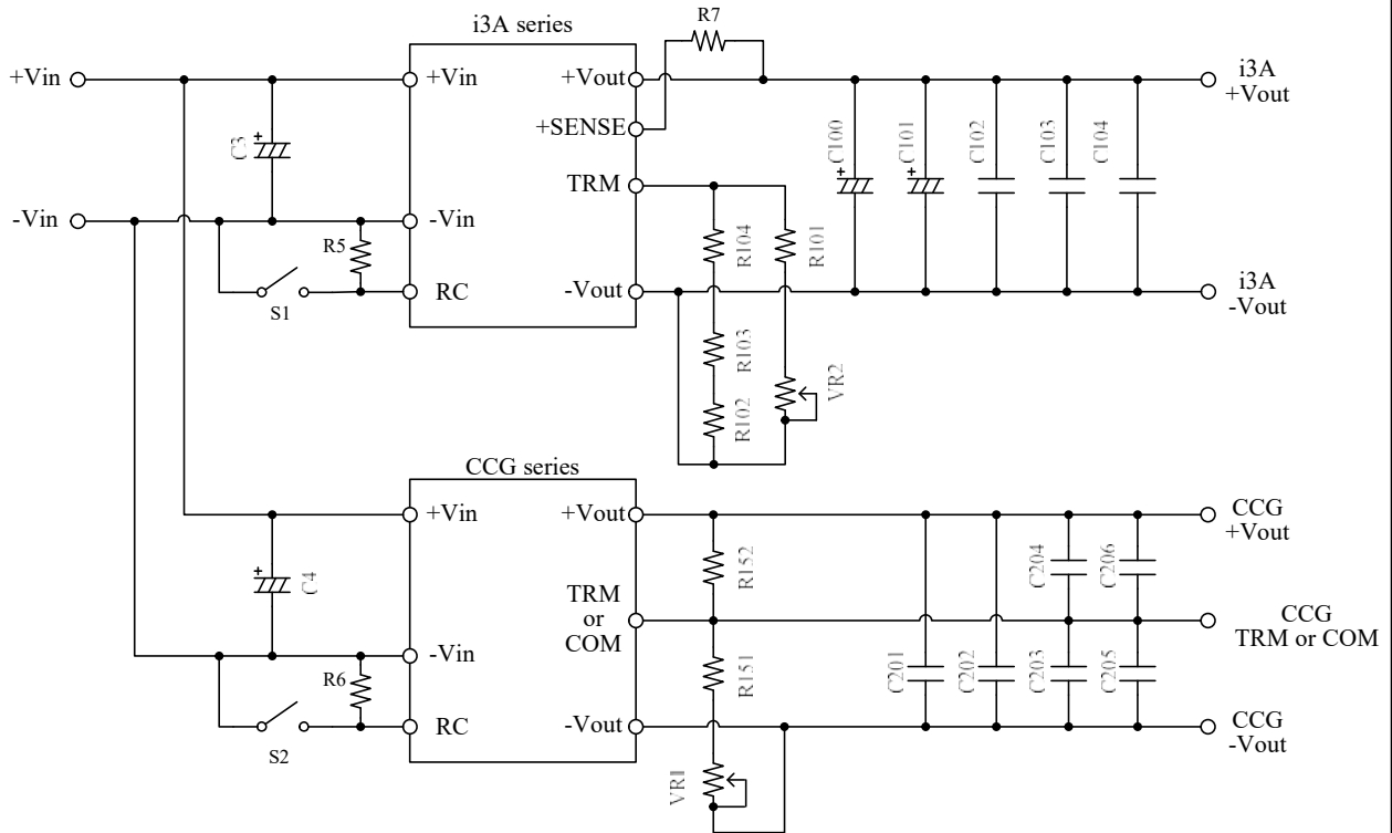
Fig.5-1 Schematic
