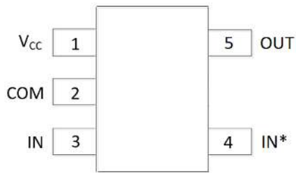
Top View TSOT25
