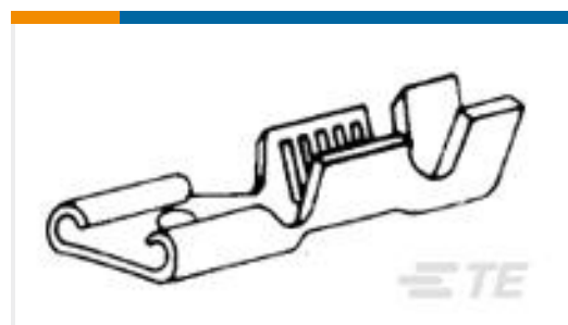
TE Part #170456-2 PL 250 AM REC 12-10 0.40 X 21 PRE- TPBR
