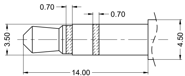
Plug
