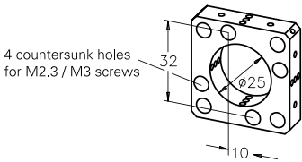
Mounting example
