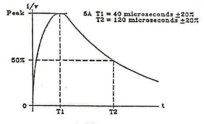
t - Time FIGURE 9 – Waveform 5A
