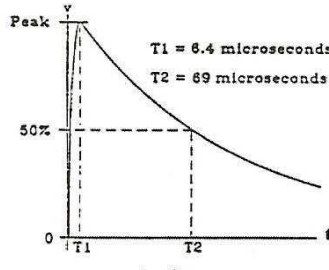
t - time FIGURE 8 – Waveform 4
