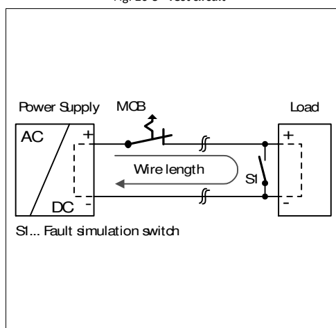
Fig. 26-5 Test circuit
