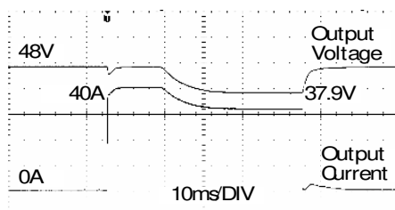
Fig. 26-3 Peak load with 2x the nominal current for 50ms, typ.
