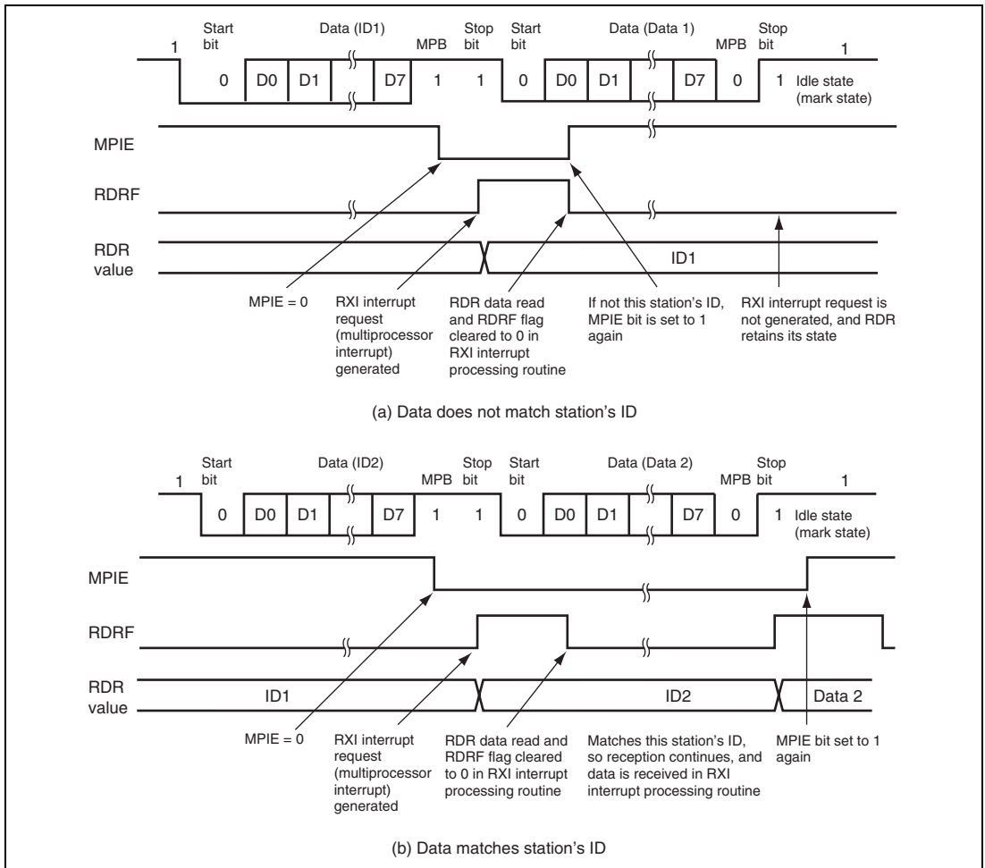
Figure 13.12 Example of SCI Operation for Reception (Example with 8-Bit Data, Multiprocessor Bit, One Stop Bit)
