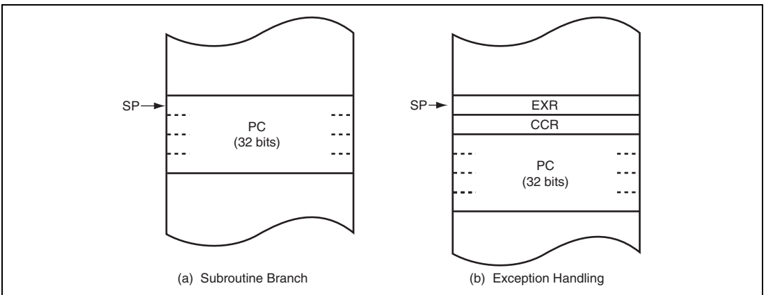
Figure 2.7 Stack Structure in Maximum Mode
