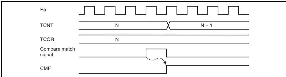
Figure 11.7 Timing of CMF Setting at Compare Match
