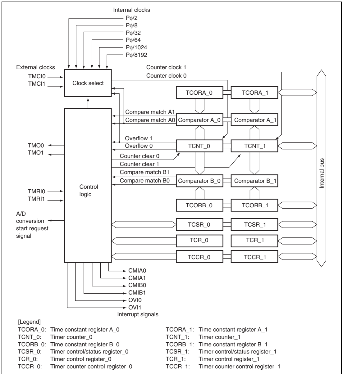
Figure 11.1 Block Diagram of 8-Bit Timer Module (Unit 0)
