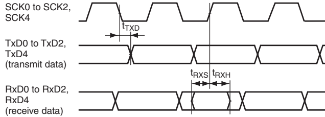
Figure 20.30 SCI Input/Output Timing: Clocked Synchronous Mode
