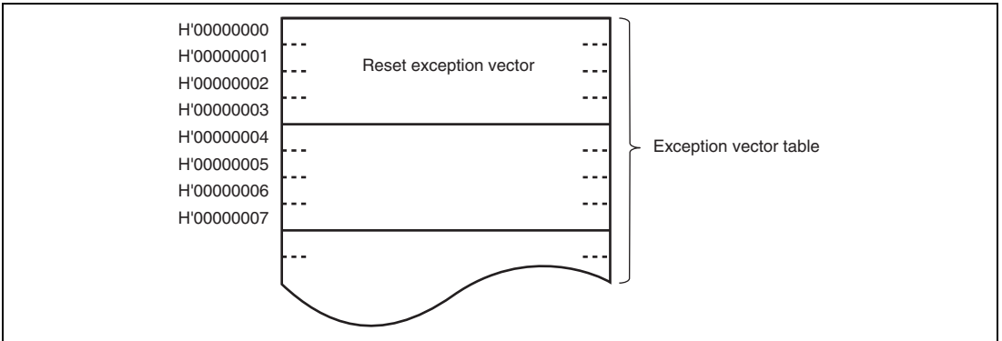
Figure 2.6 Exception Handling Vector Table (Maximum Modes)
