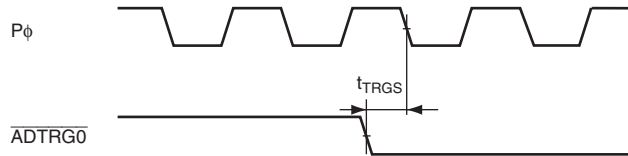
Figure 20.31 A/D Converter External Trigger Input Timing
