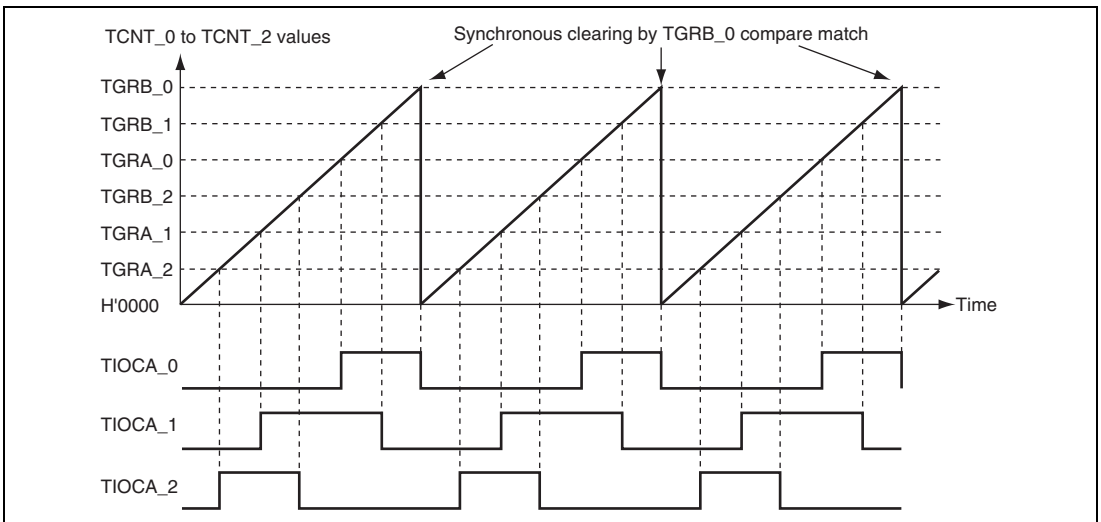
Figure 9.11 Example of Synchronous Operation
