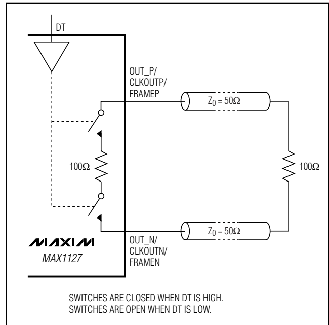
Figure 8. Double Termination
