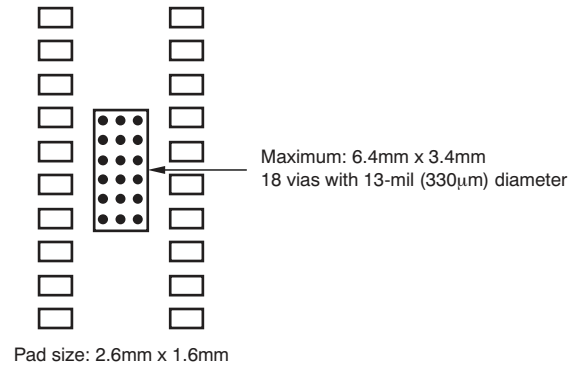
Figure 1. Land Pattern
