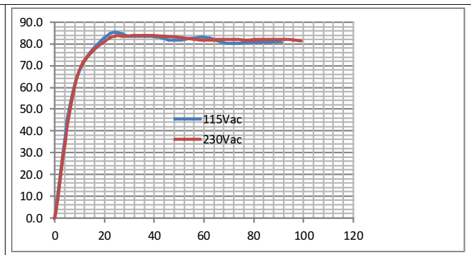
Figure 6. Efficiency 12.5-V Buck Boost
