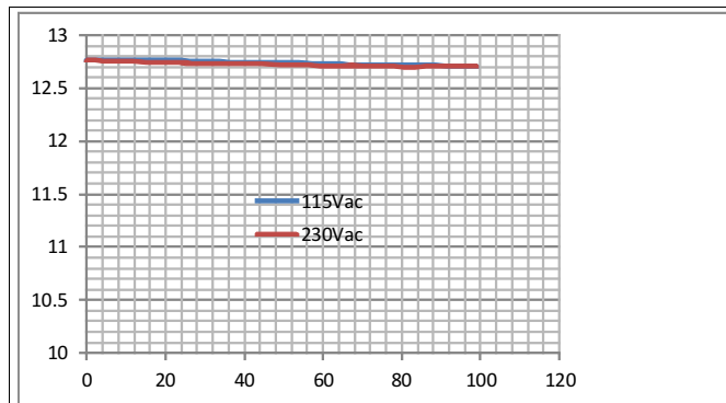
Figure 5. Regulation 12.5-V Buck Boost
