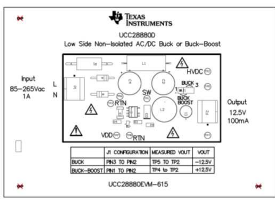
Figure 10. UCC28880EVM-615 Layout (top layer)
