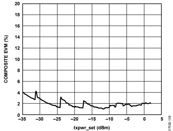
Figure 9. TXLBRF, UMTS Band V, Transmit EVM vs. tppwr_set (dBm), Four Calibration Points Applied, Transmit Frequency 881 MHz.
