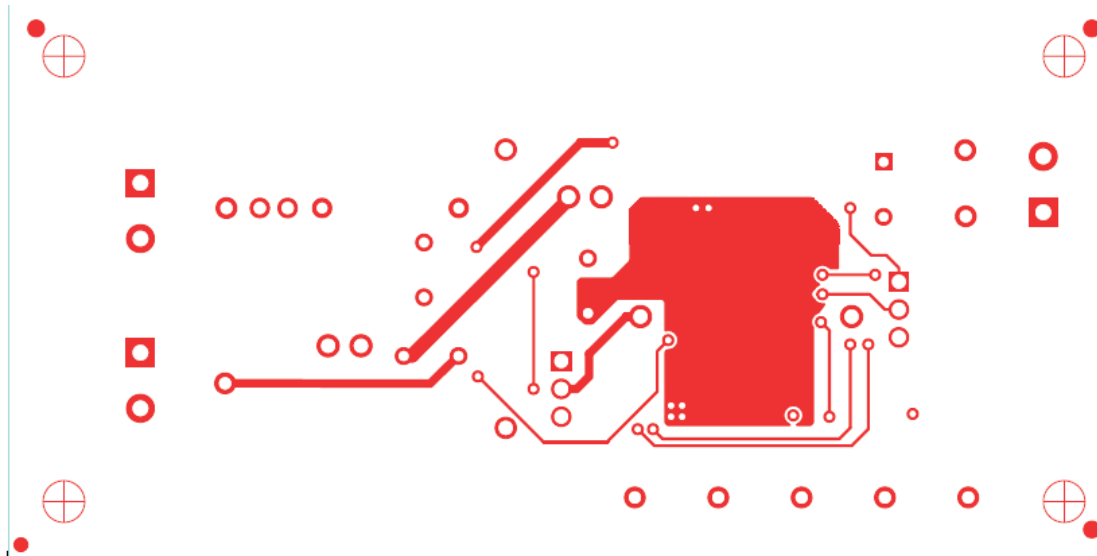
Figure 31. Top Copper (top view)
