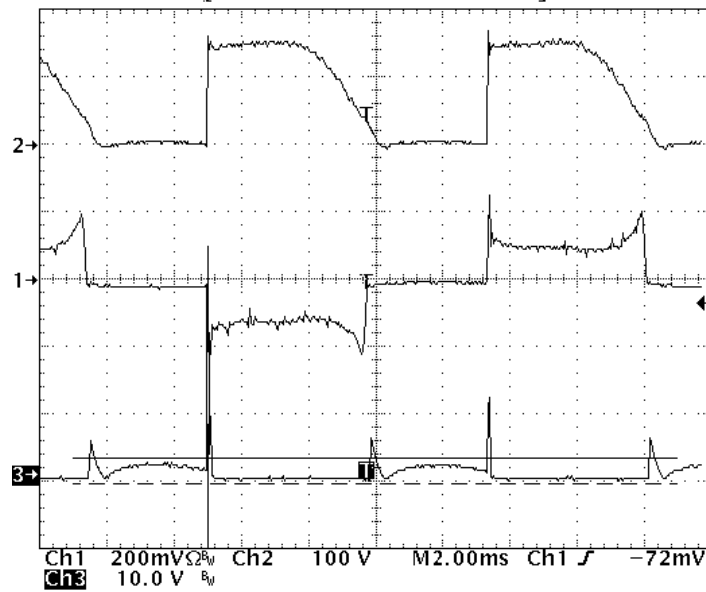
Figure 19. Dummy Load Conduction Time vs. Dimmer Setting (Ch1- line current Ch2- bulk voltage Ch3- Q4 source voltage)
