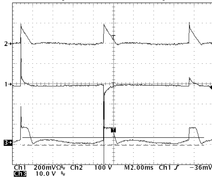
Figure 15. Dummy Load Conduction Time vs. Dimmer Setting (Ch1- Line current Ch2- bulk voltage Ch3- Q4 source voltage)
