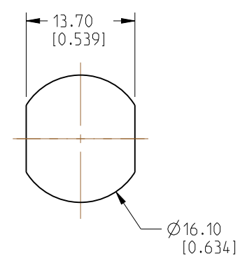
RECOMMENDED MOUNTING HOLE DIMENSIONS
