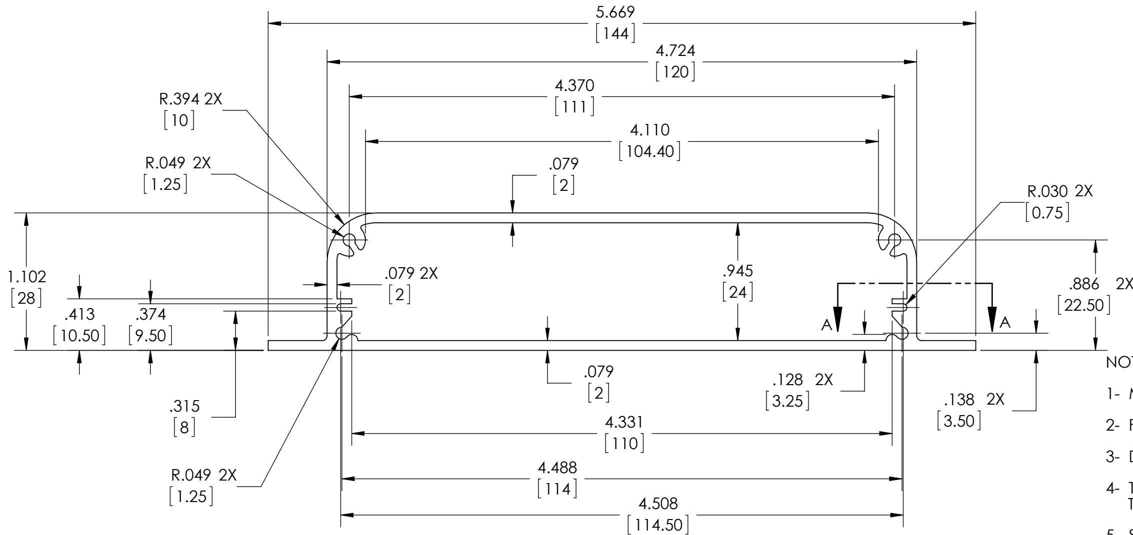
EXTRUSION PROFILE
