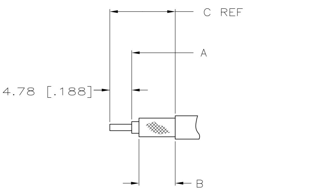
RECOMMENDED STRIP LENGTH FOR STANDARD COAX CABLE
