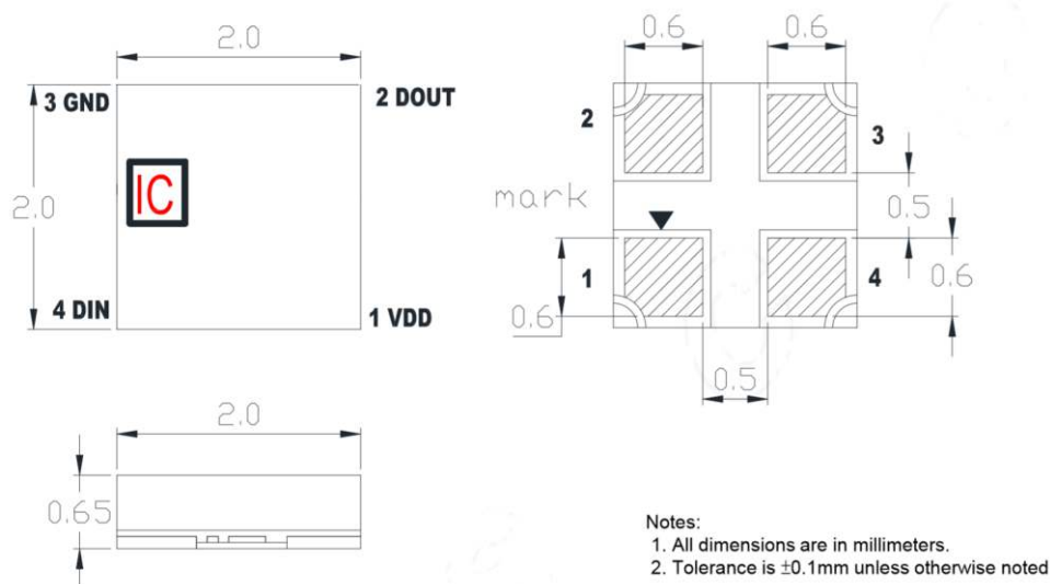
Figure 1. IN-PI20TAT(X)R(X)G(X)B Package Outline Dimensions
