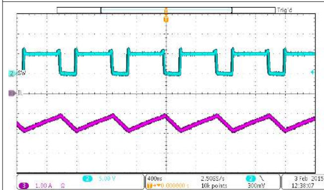
Figure 9-12. Boost Mode Switching Waveform
