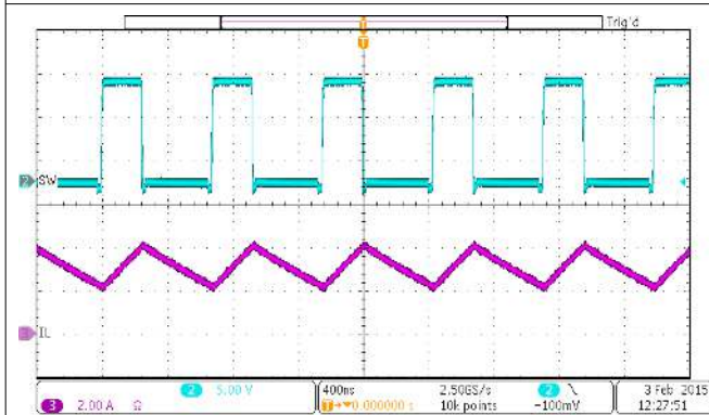
Figure 9-10. PWM Switching Waveform
