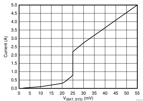
Figure 8-4. BATFET V-I Curve
