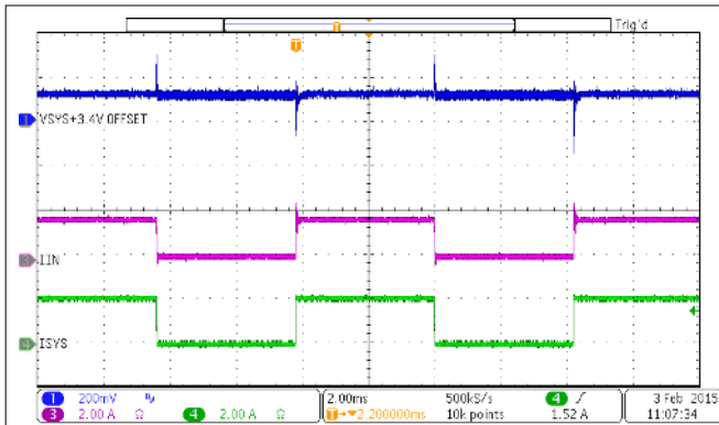
Figure 9-8. Input Current DPM Response without Battery
