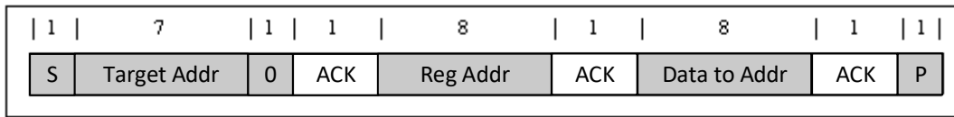
Figure 8-13. Single Write
