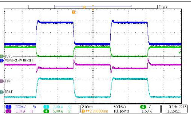
Figure 9-9. Load Transient During Supplement Mode
