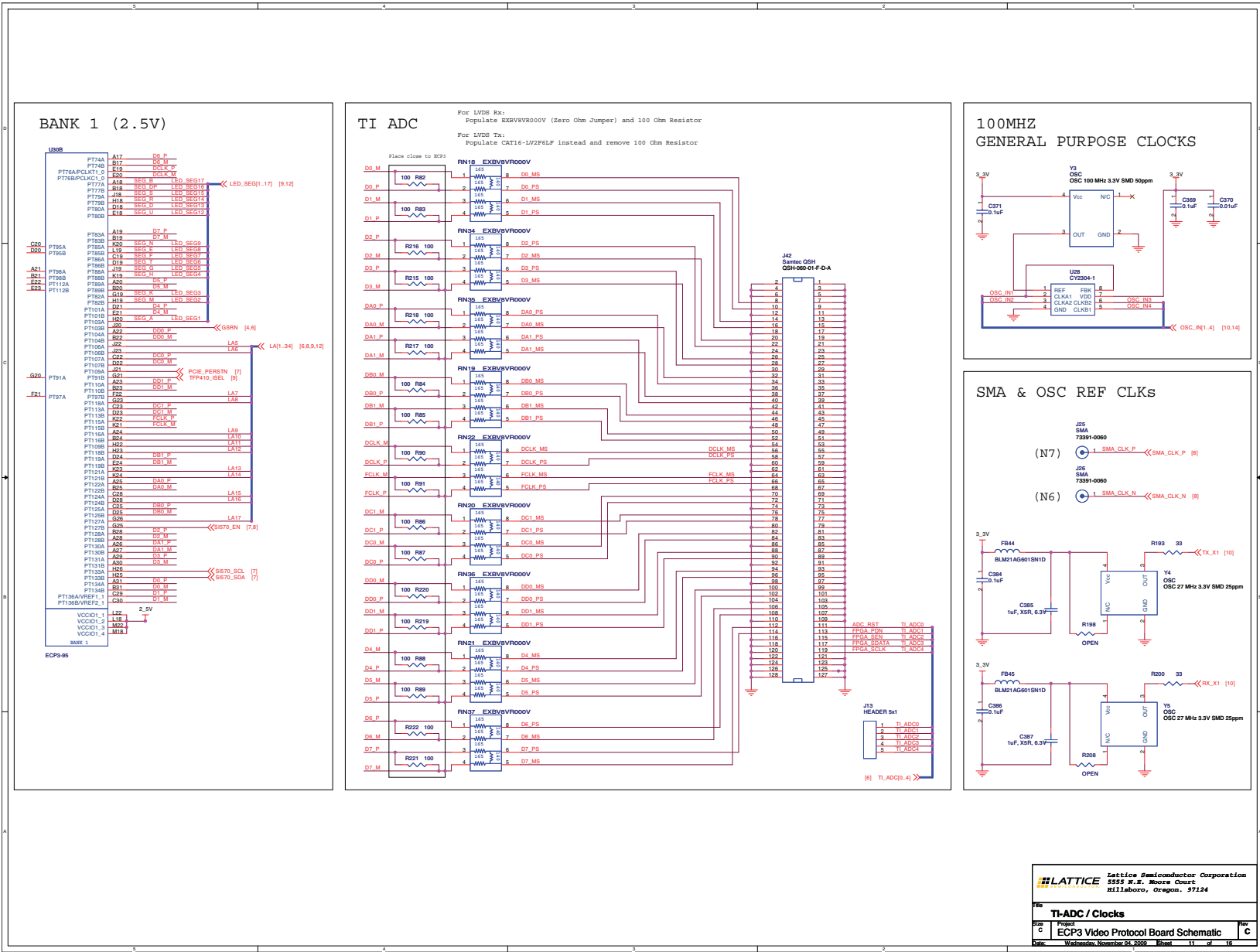
Figure 20. TI-ADC/Clocks
