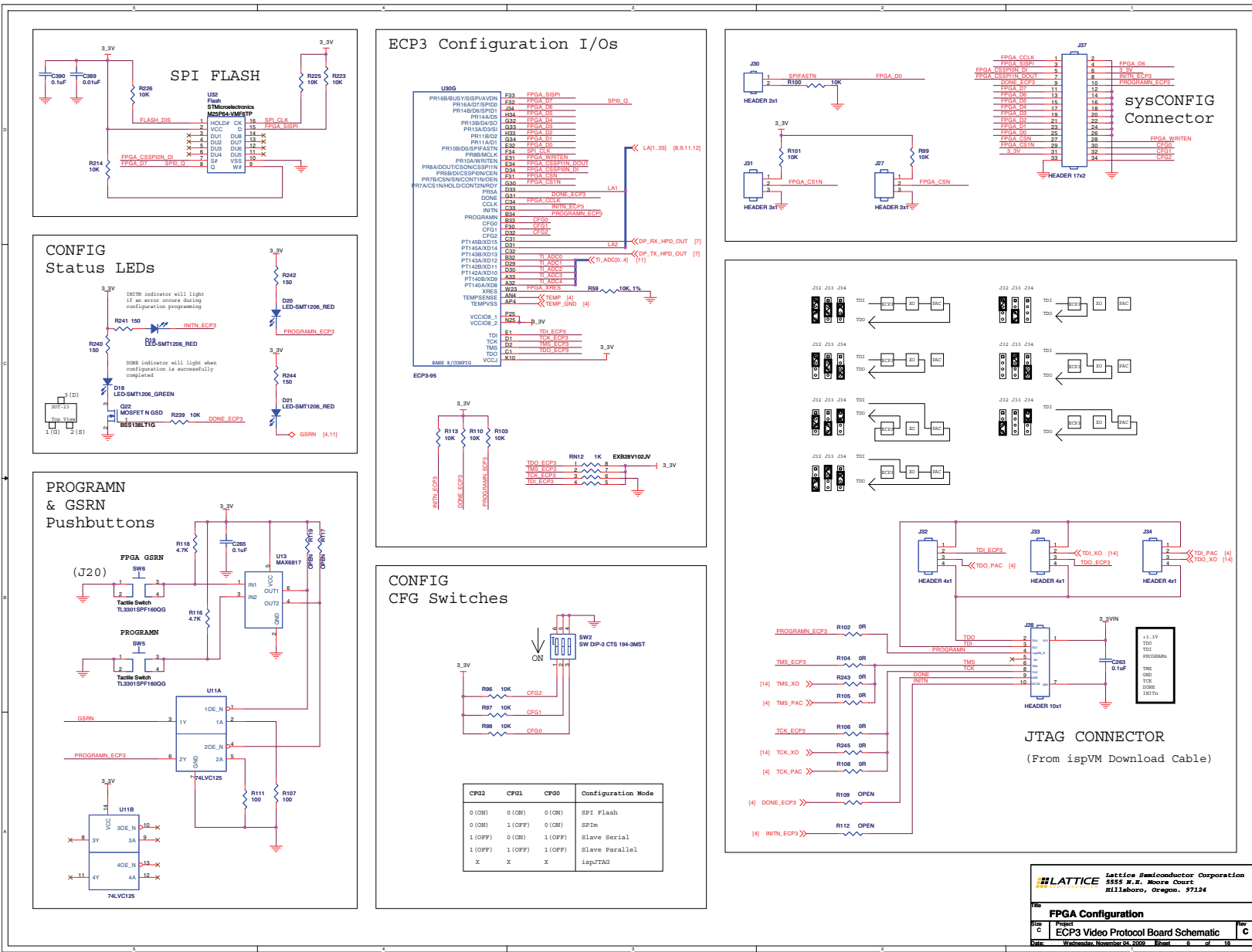
Figure 15. FPGA Configuration
