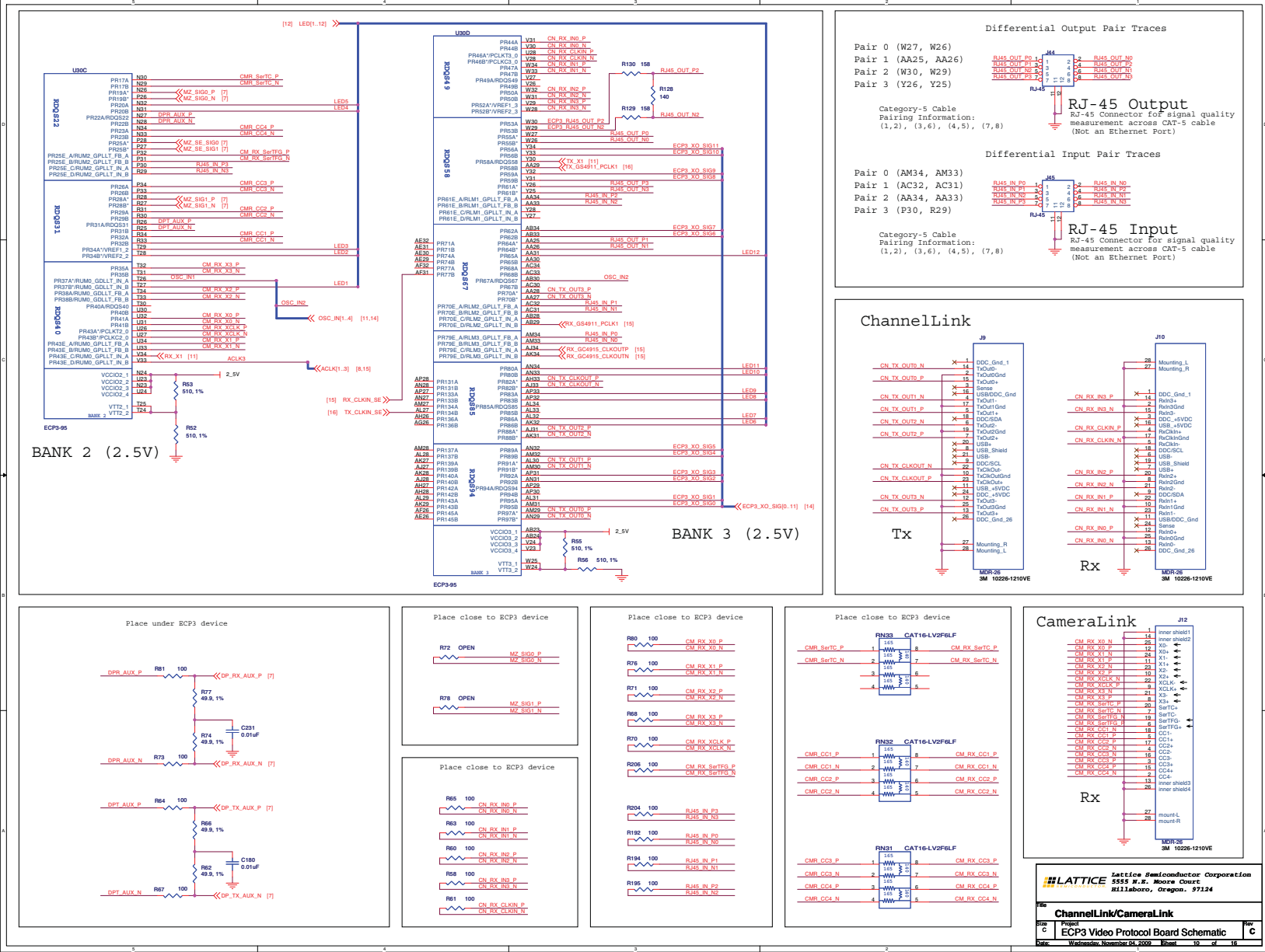
Figure 19. ChannelLink/CameraLink
