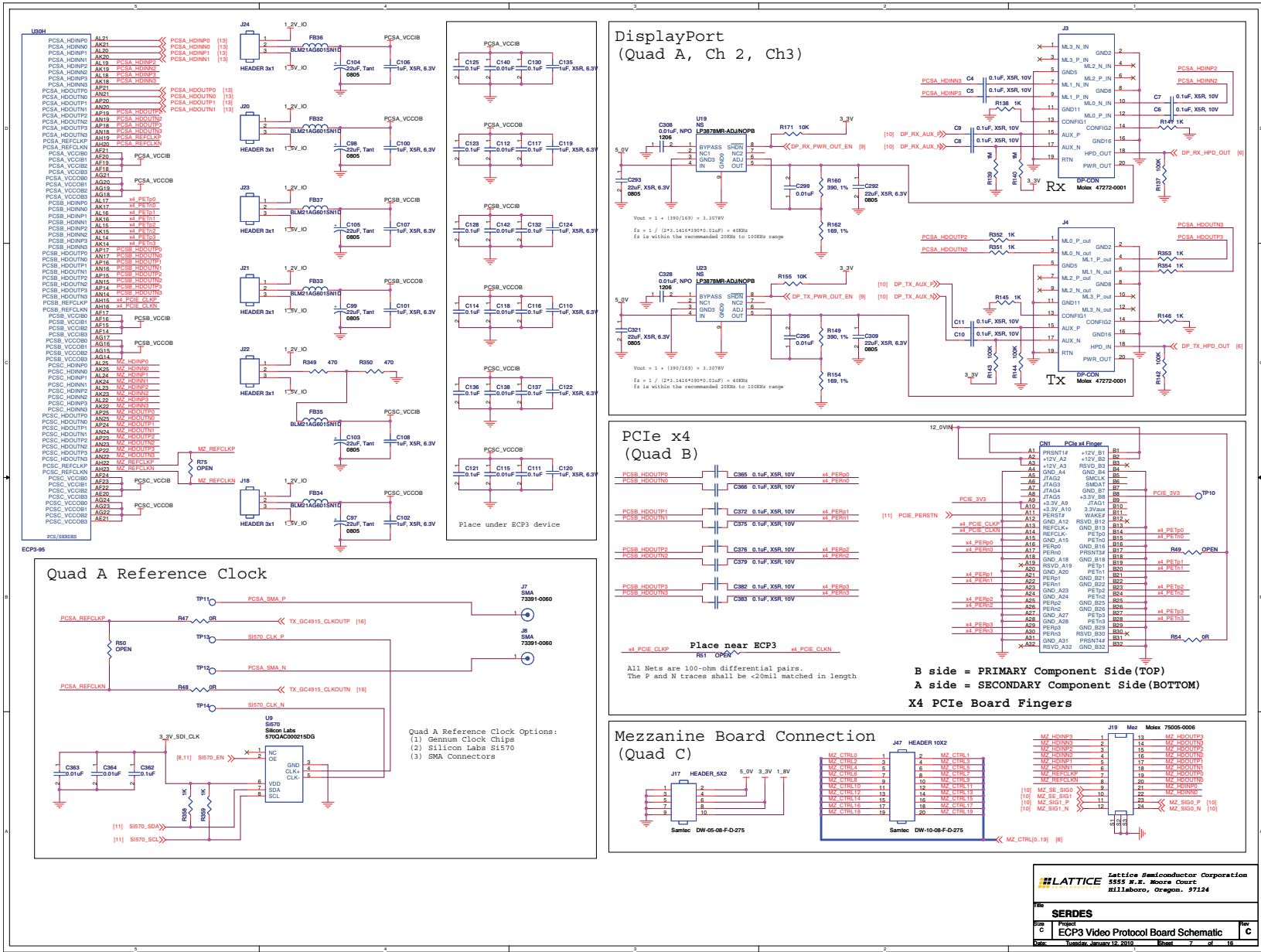
Figure 16. SERDES
