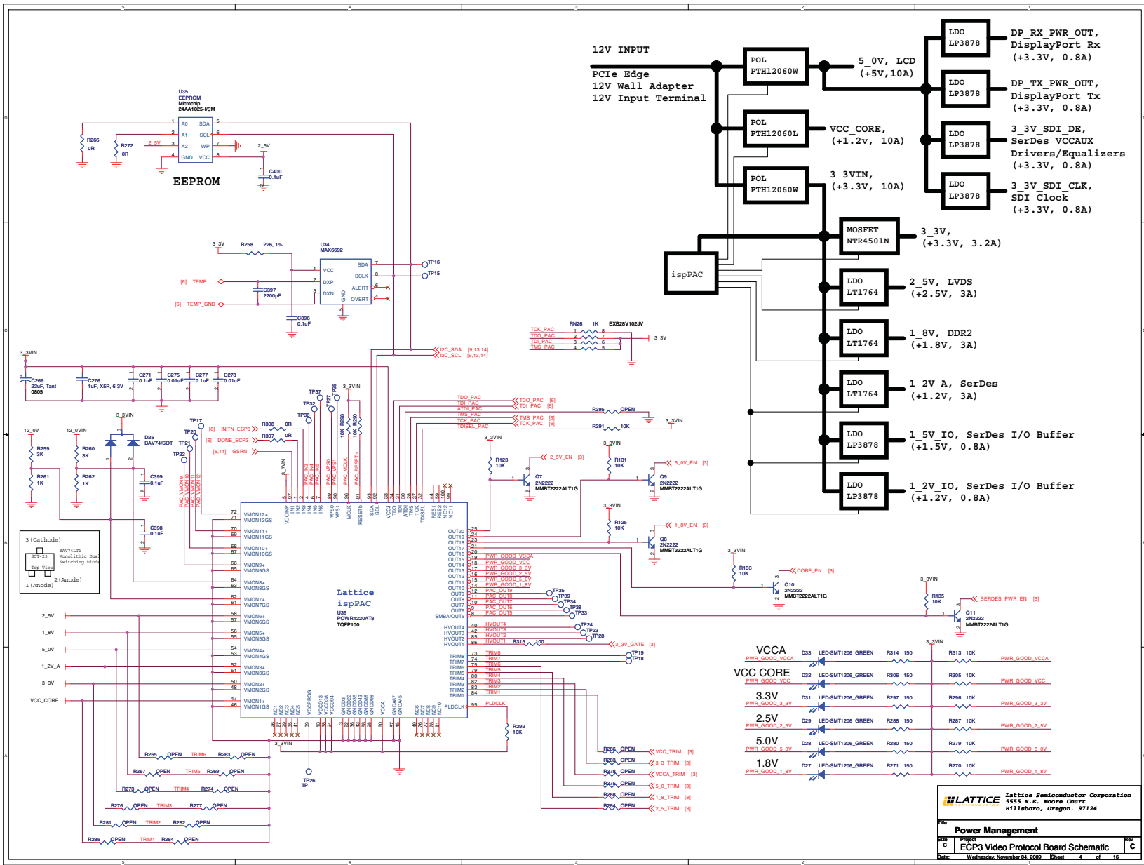
Figure 13. Power Management
