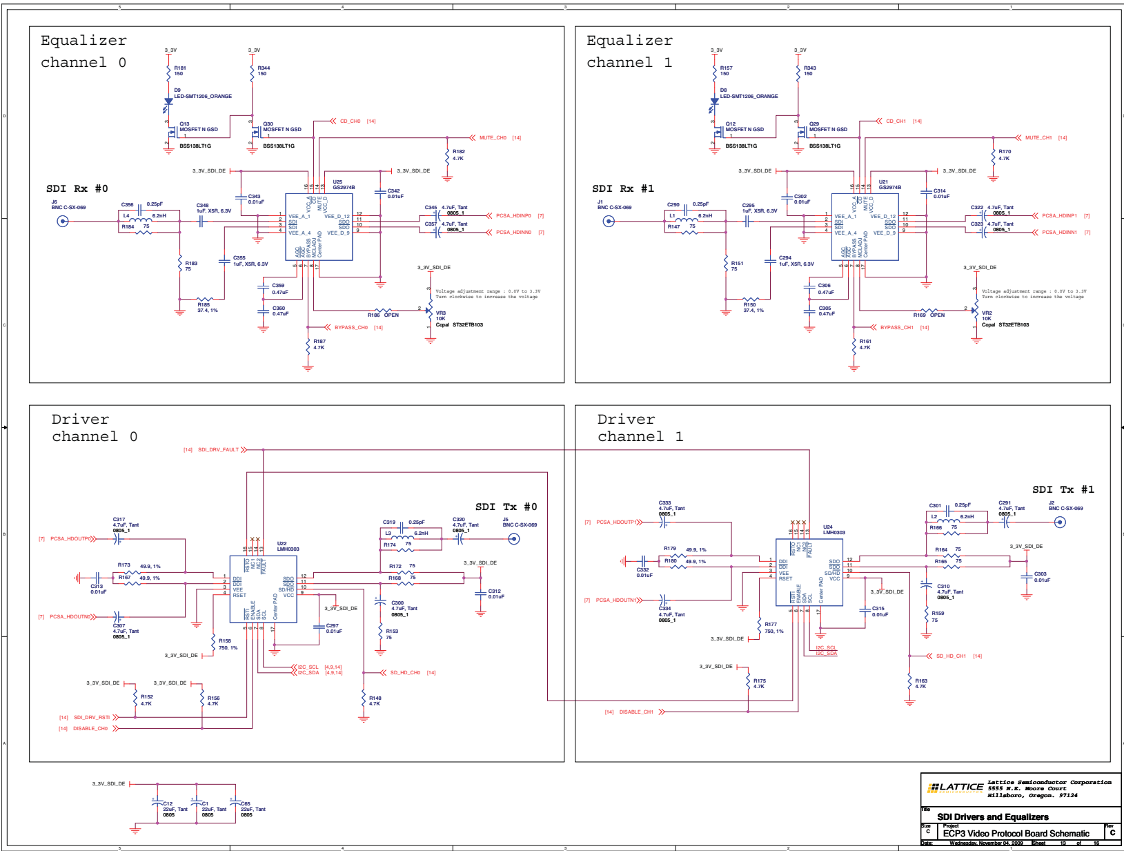
Figure 22. SDI Drivers and Equalizers
