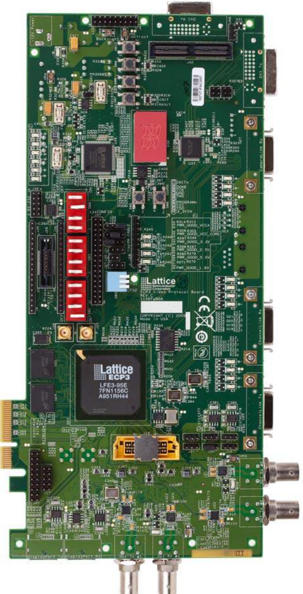
Figure 1. LatticeECP3 Video Protocol Board – Revision C
