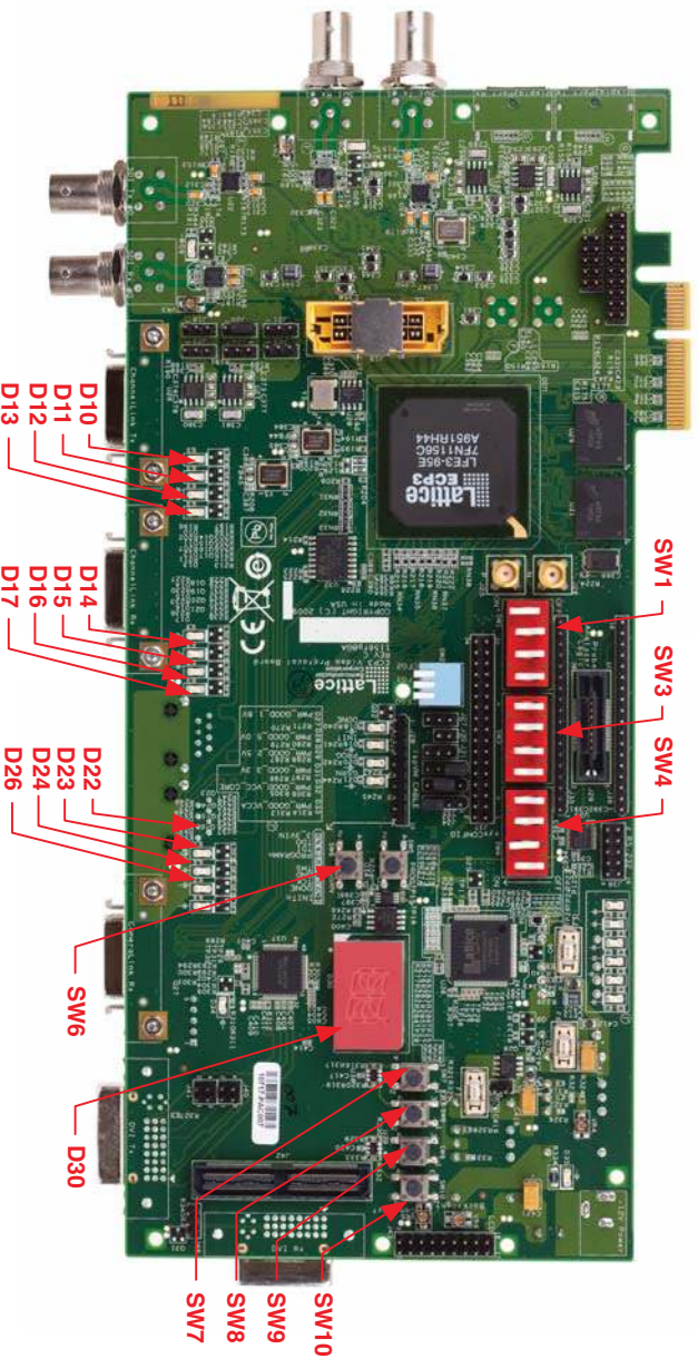
Figure 9. Switch and LED Locations
