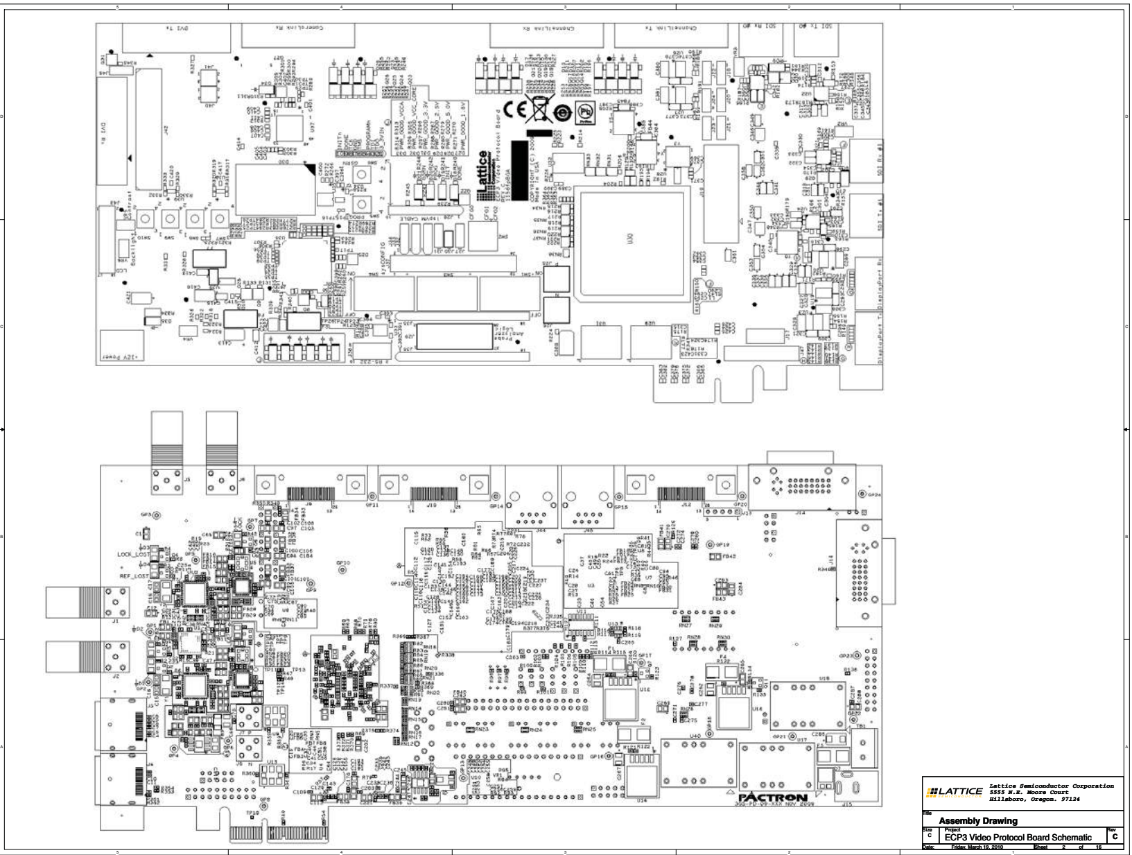
Figure 11. Assembly Drawing
