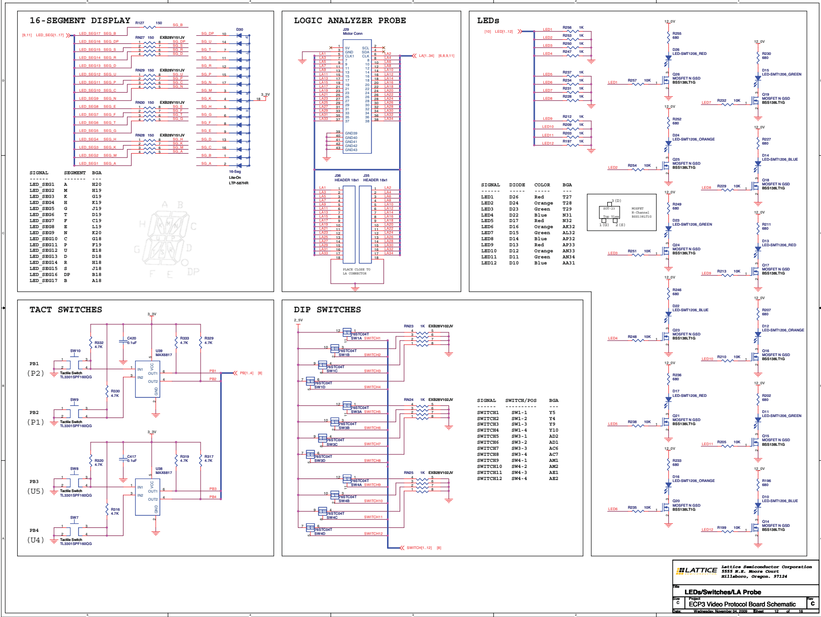
Figure 21. LEDs/Switches/LA Probe
