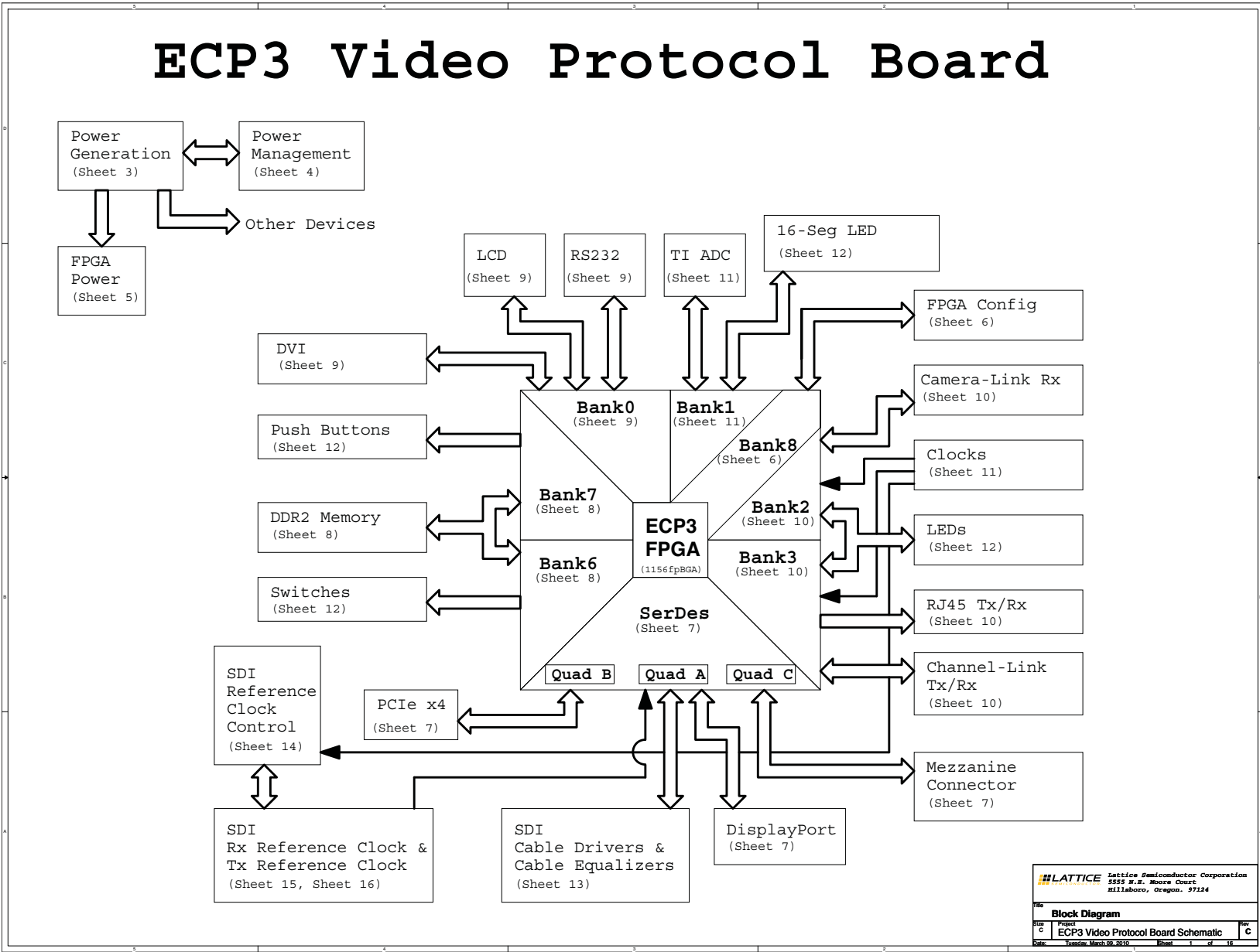
Figure 10. Block Diagram
