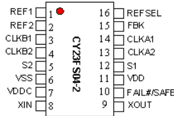
Figure 1. 16-Pin TSSOP
