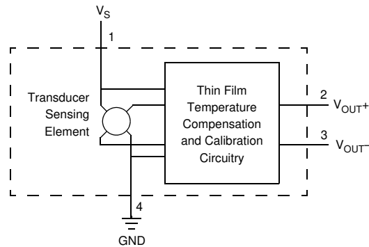
Figure 1. Block diagram
